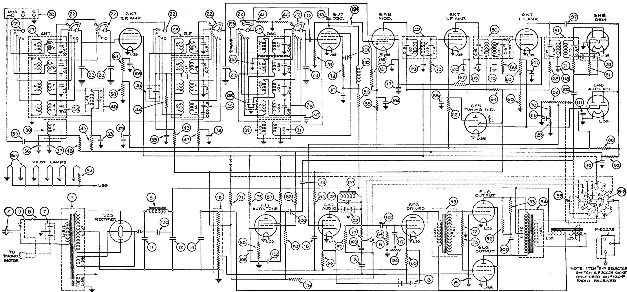
Fig. 2. Schematic Circuit of Receiver.
